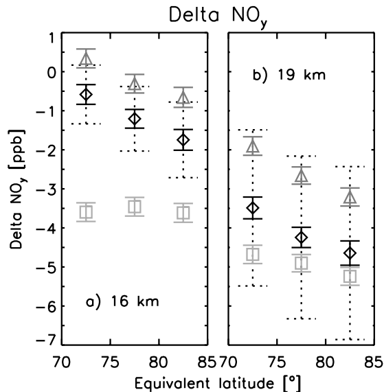
Figure 5. Average denitrification for regions between 85^\circ and 80^\circ , between 80^\circ and 75^\circ as well as between 75^\circ equivalent latitude and the vortex edge for 16 km altitude (a) and for 19 km altitude (b) in mid-March. The diamonds show denitrification derived from measurements, with the solid error bars giving the standard deviation about the mean and the dotted error bars giving the full accuracy. The triangles show results from the SLIMCAT ice run, while the squares show results from the SLIMCAT NAT run, with the error bars giving the standard deviation about the mean in each case.
